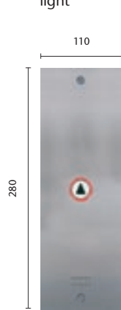
KSL 210: Round grey buttons with amber call acceptance light
